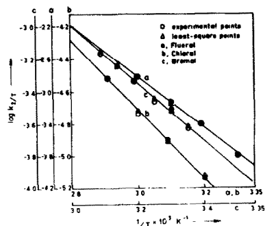
Figure 8 Plots of \log k_2/T against 1/T
